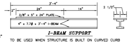
TYPE "C" FOR INLET DESIGN NO. 3
